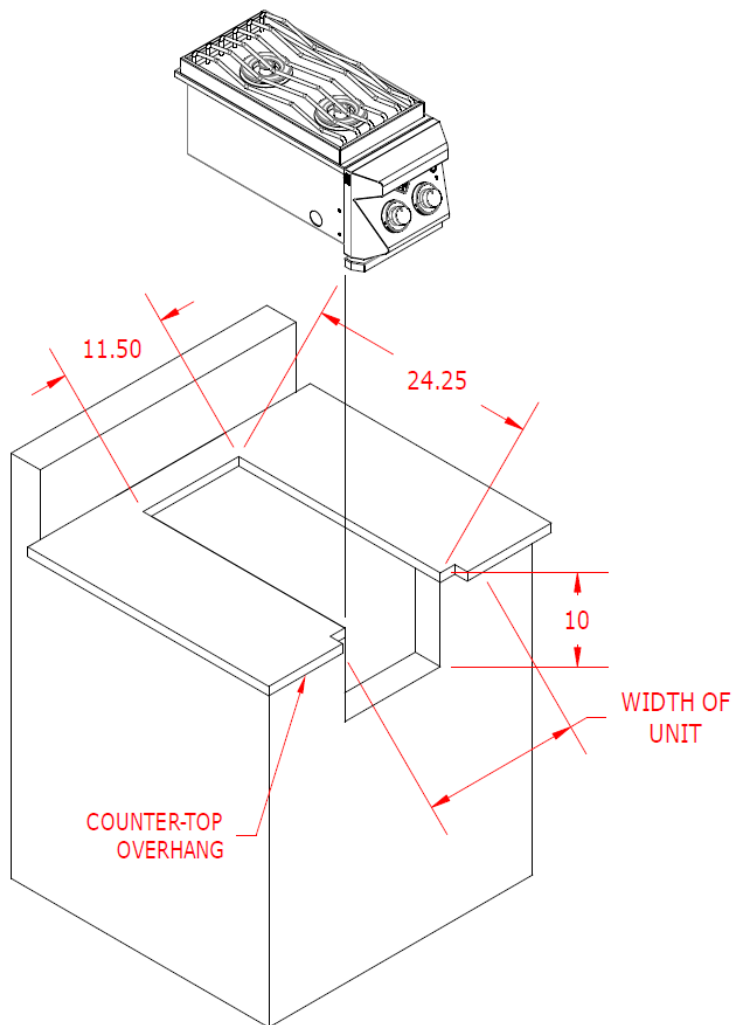
TYPICAL SIDE BURNER INSTALLATION INTO NON- COMBUSTIBLE CONSTRUCTION
